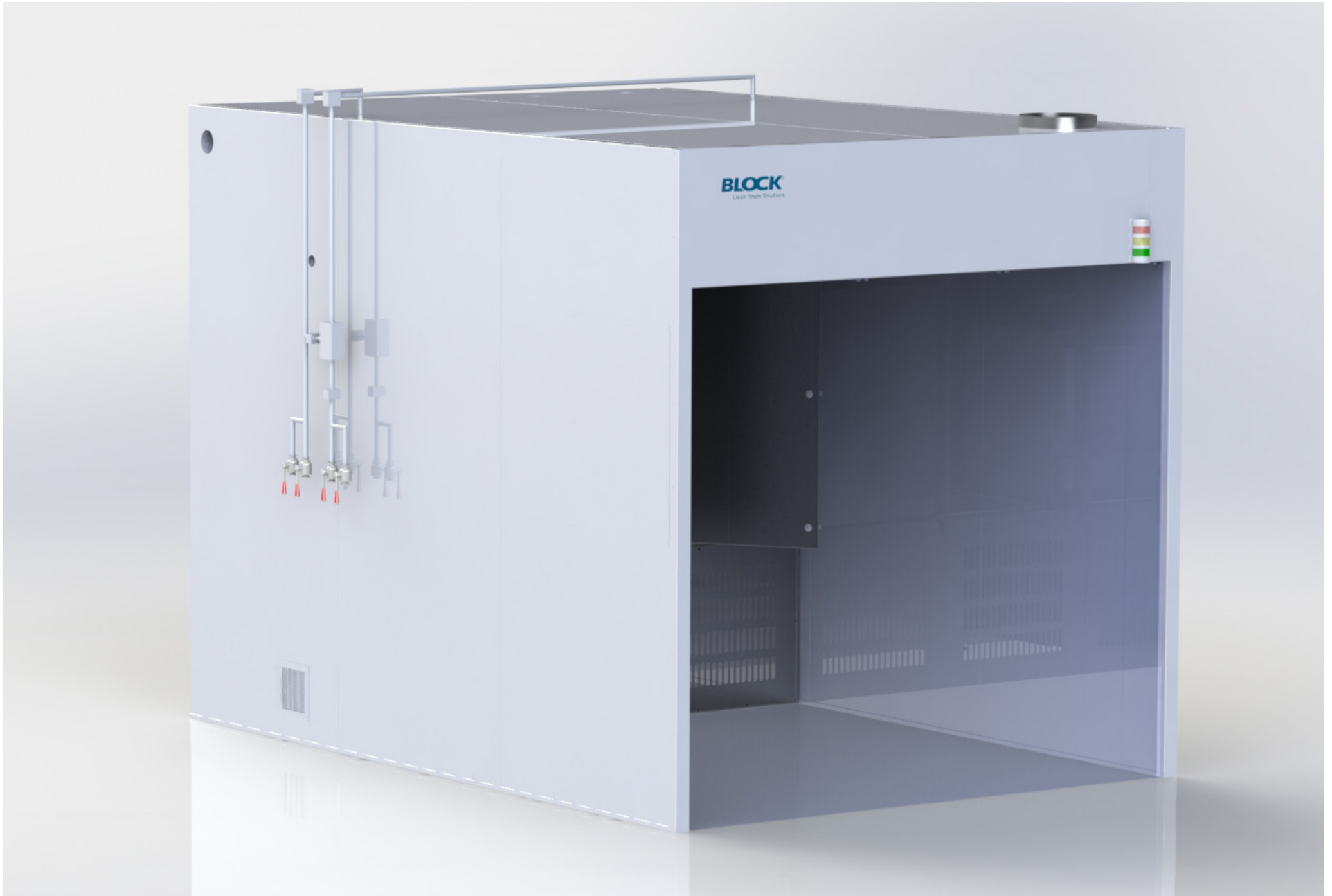
Weighing box for weighing loose materials and consists of a working and an installation space | Teva Czech Industries s.r.o., Opava | Czech Republic
